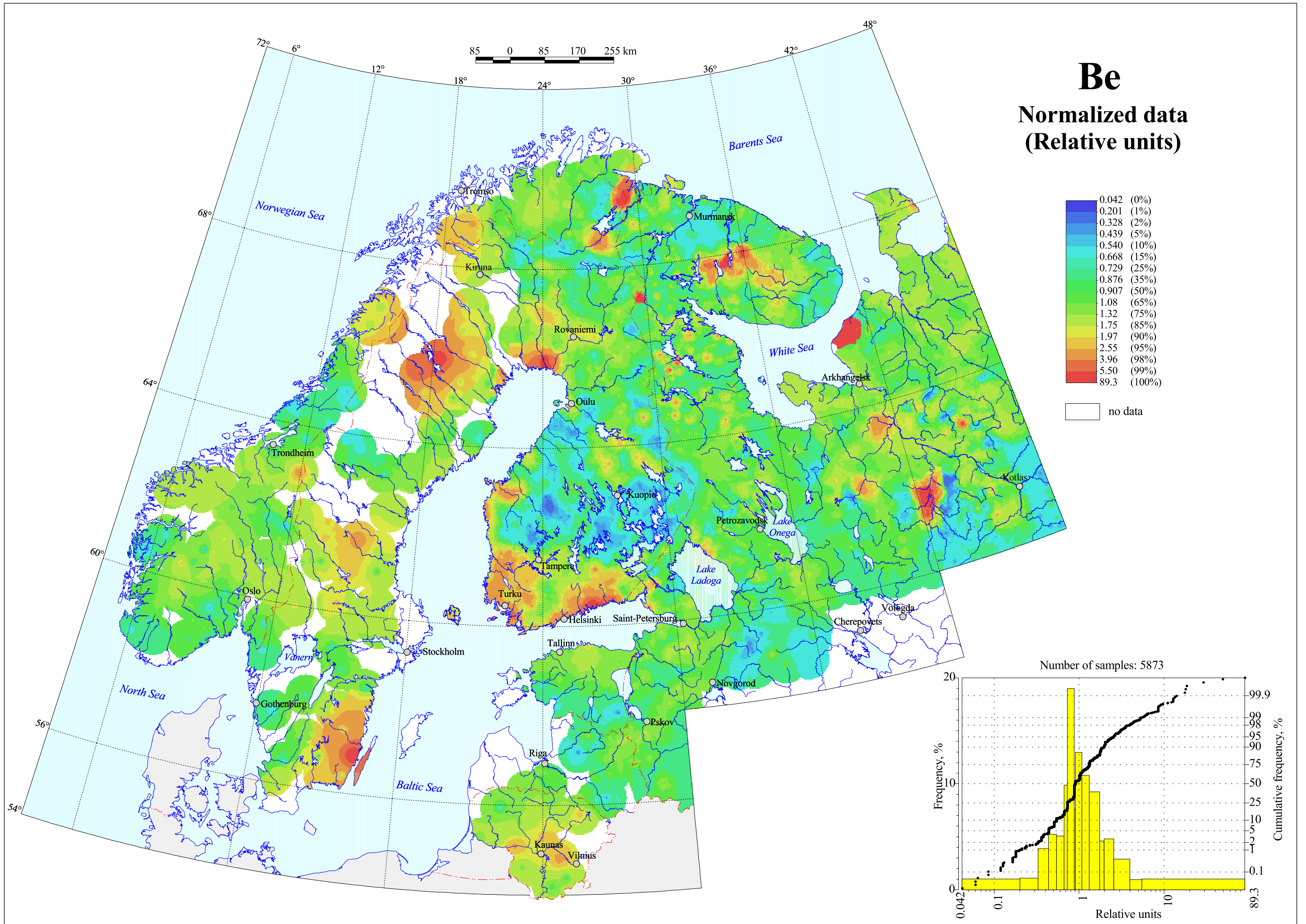
Beryllium in Stream Sediment
